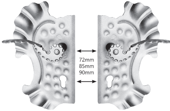
3444100 160x290mm 2mm
