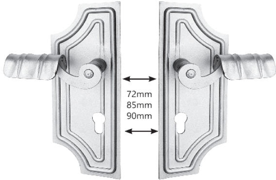
3443600 104x277mm 2mm
